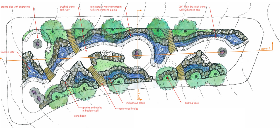
Overall Plan of Rain Garden Scale: 1" = 80'-0"
